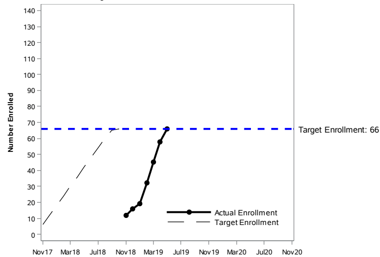
Kenya: Kisumu: Kisumu CRS Total Enrollment = 66
