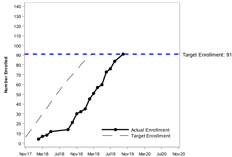
Botswana: Gaborone: Gaborone CRS Total Enrollment = 91
